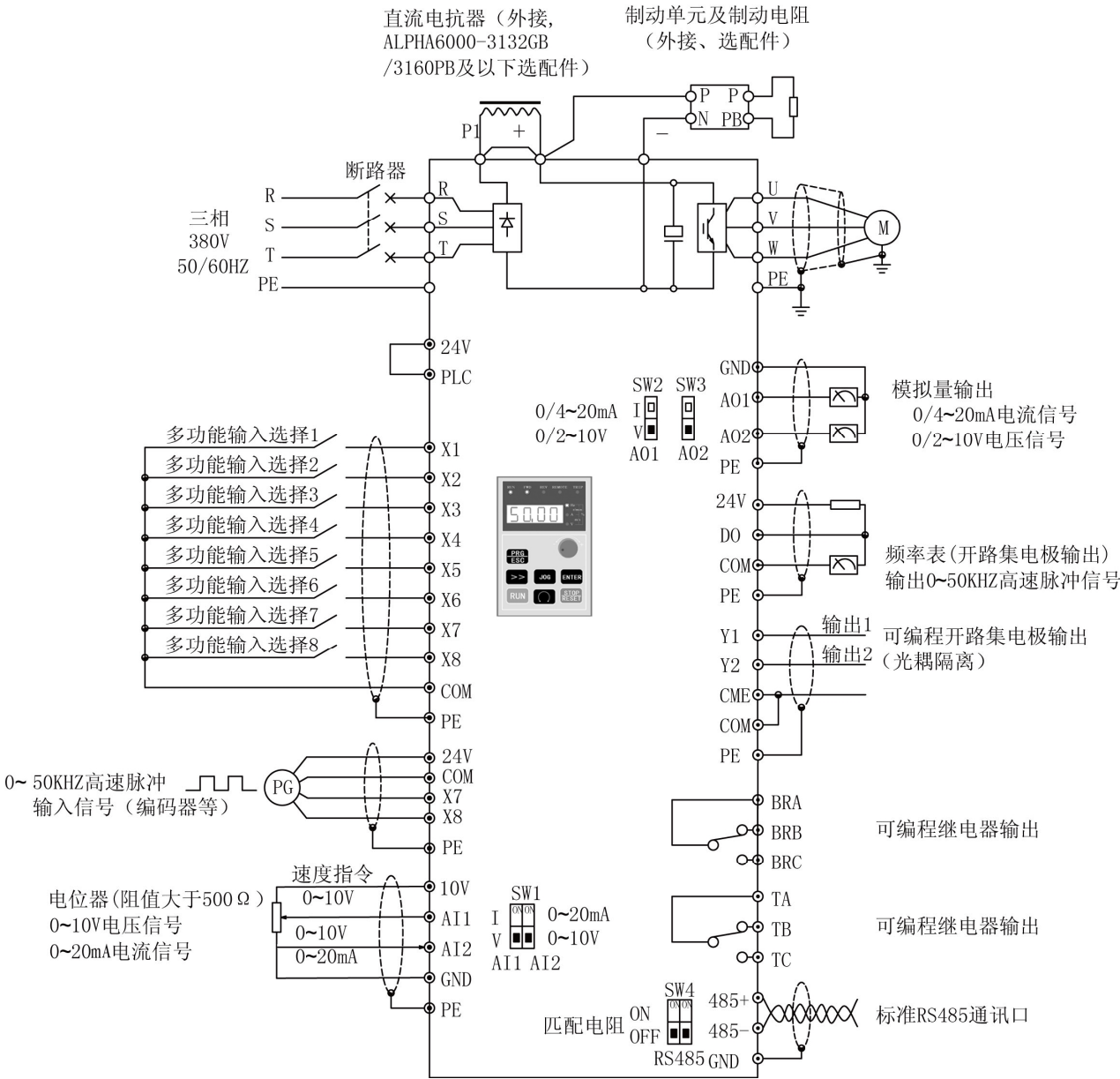
图 2-26 3018G/3022P~3355G/3400P~3500G接线图
